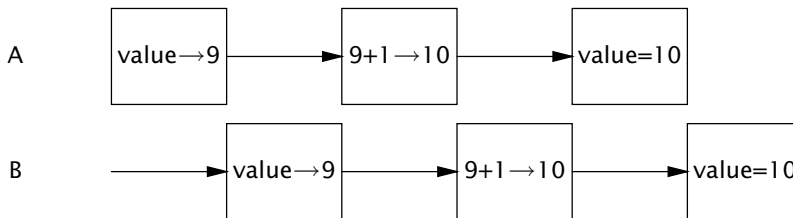
FIGURE 1.1. Unlucky execution of UnsafeSequence.nextValue .
