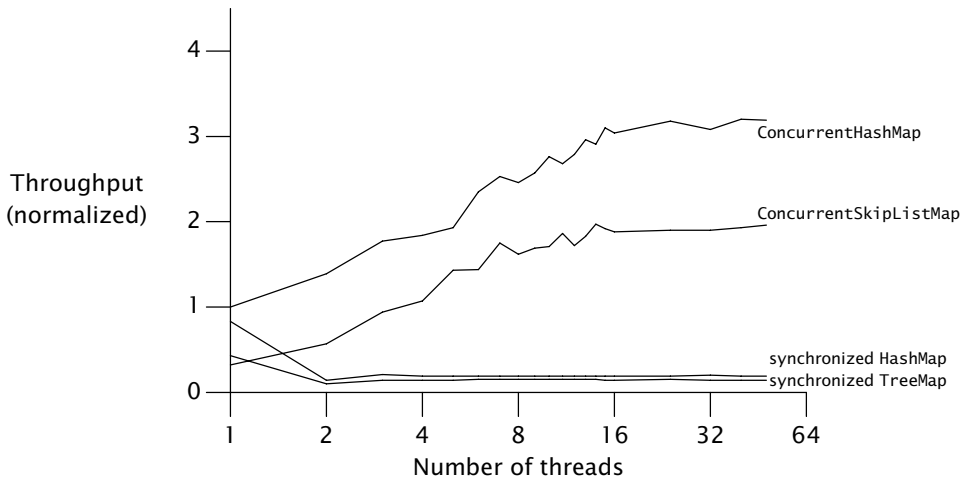
FIGURE 11.3. Comparing scalability of Map implementations.
