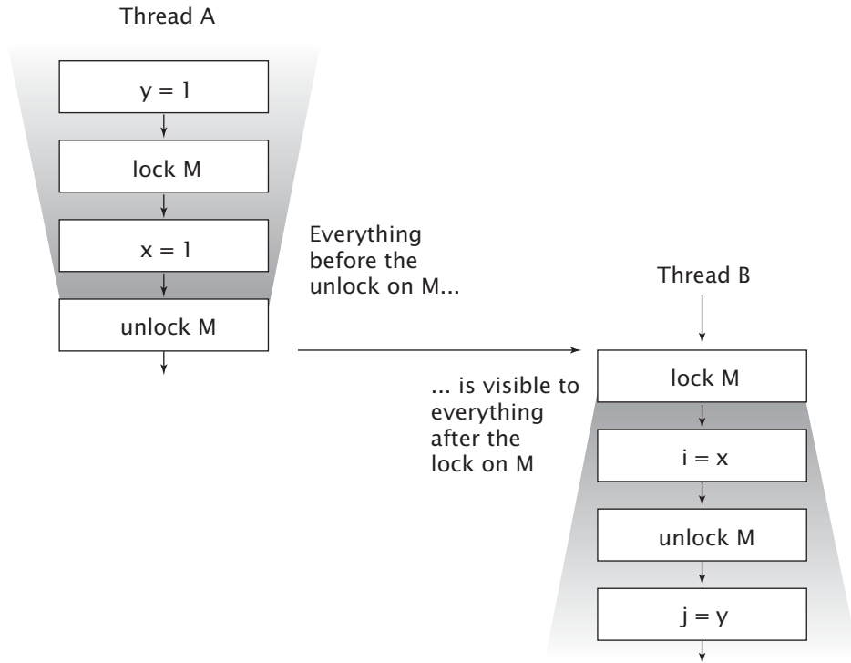
FIGURE 3.1. Visibility guarantees for synchronization.
